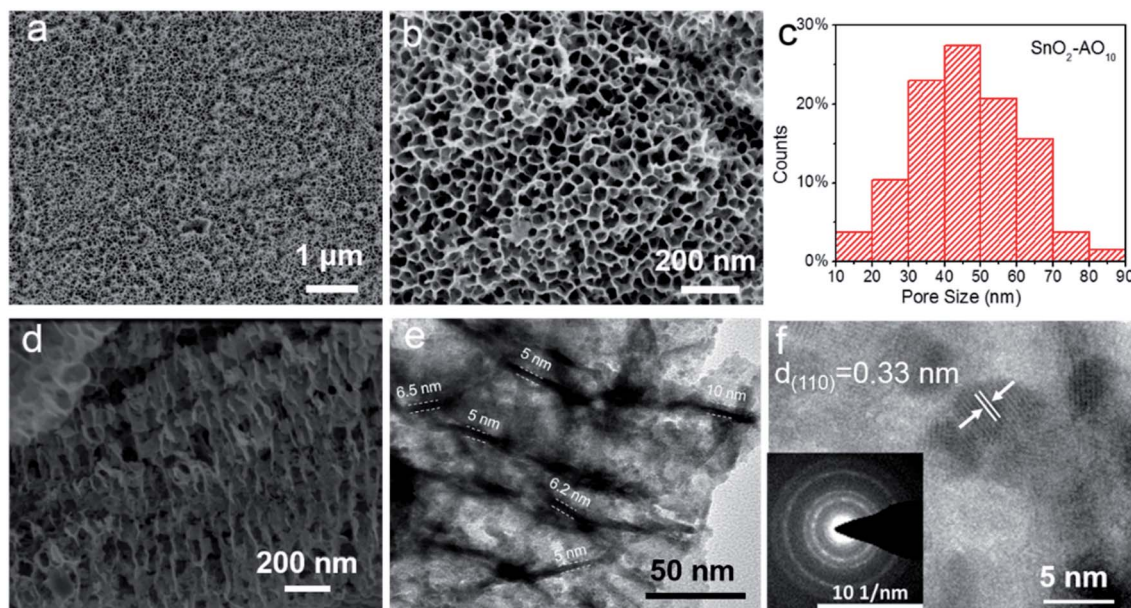
Fig. 2 (a and b) SEM images and (c) the corresponding pore size statistical analysis of the surface of SnO 2 -AO 10 . (d) SEM and (e) TEM images of the cross-section of SnO 2 -AO 10 . (f) High-resolution TEM image and the corresponding electron diffraction pattern (inset) of SnO 2 -AO 10 .
