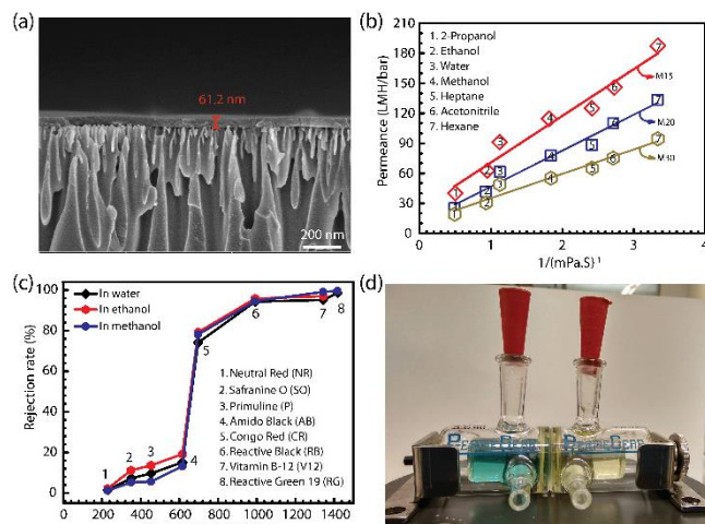
Figure 4: (a) Cross-section SEM image of sample M20; (b) Permeances of water and a number of polar and non-polar organic solvents through the three TFP-DHF 2D COF membranes with 15 (M15), 20 (M20), and 30 (M30) layers are plotted with the inverse of their viscosity; (c) Rejection rates of various dyes through the M20 membrane vs. their molecular weight; (d) Image showing the separation of the mixture dyes of Reactive Green (RG) and Primuline (P). The chamber on the left-hand side contains the mixture of the two dyes, whereas the chamber on the right-hand side is filled with fresh water initially and turned yellow after 1-day diffusion.
