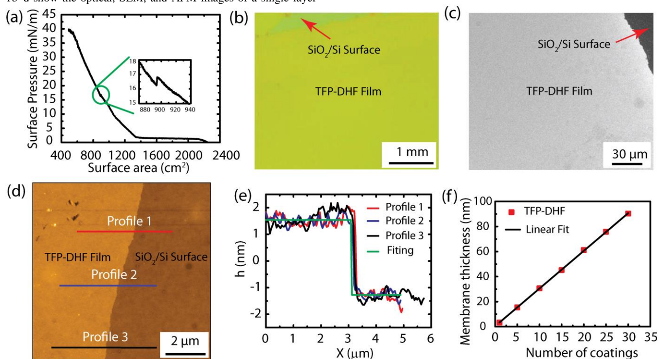
Figure 1. Membrane characterization (a) Surface-pressure-area isotherm, a step was observed at surface pressure of 17 mN/m, and the polymerization was initiated at this surface pressure; (b) Optical microscopy image; (c) SEM image; (d) AFM topography image; (e) AFM height profiles of a single layer TFP-DHF film deposit on \text{SiO}_2/\text{Si} surface, the AFM profiles were calculated using the Gwyddion software; and (f) Membrane thickness at different numbers of coatings
