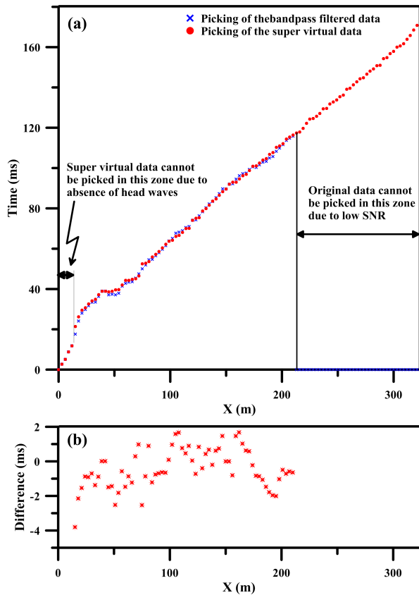
Figure 3: Graph comparing both raw data and super-virtual data picks for one shot gather.
