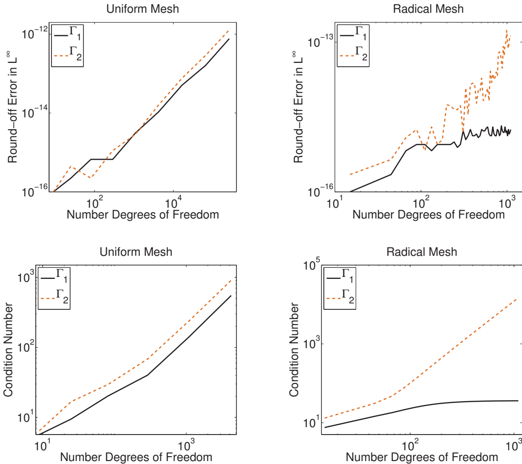
Figure 5: Log-Log representation of condition number and round-off error for 2D Laplace problem discretized with uniform grid (left) and radical mesh (right). ILP shape functions of order p = 2 are used.
