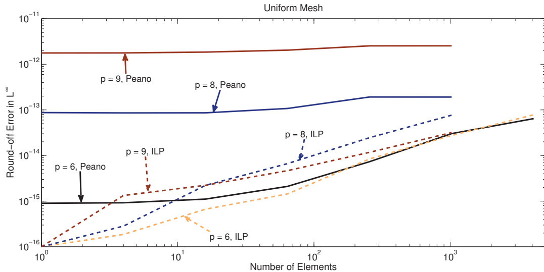
Figure 6: Round-off error for 2D Laplace problem discretized with uniform mesh.
