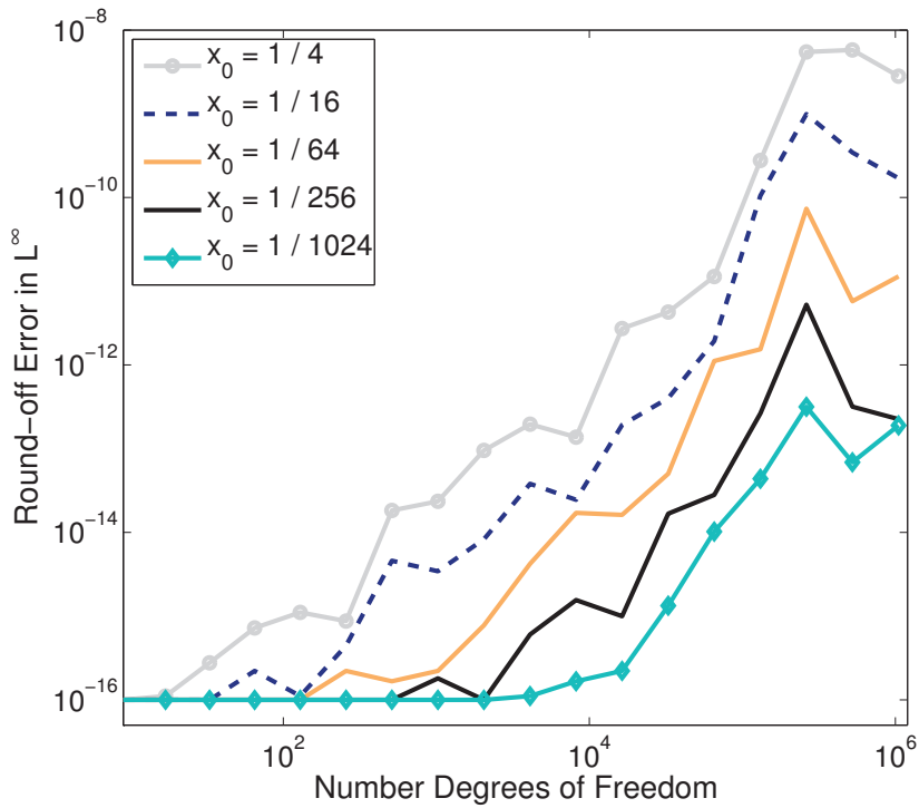
Figure 4: Round-off error for 1D Poisson problem discretized with uniform mesh. ILP shape functions of order p = 1 are used.
