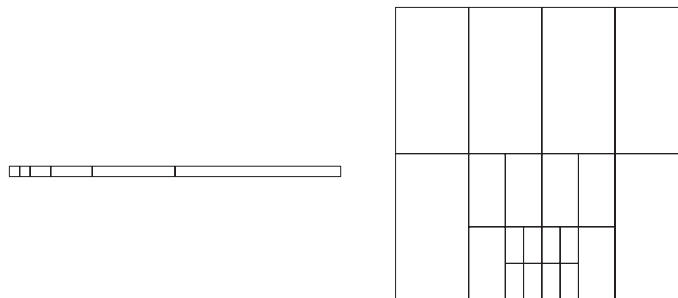
Figure 1: Left: Radical Mesh in 1D. Right: Radical Mesh in 2D.
