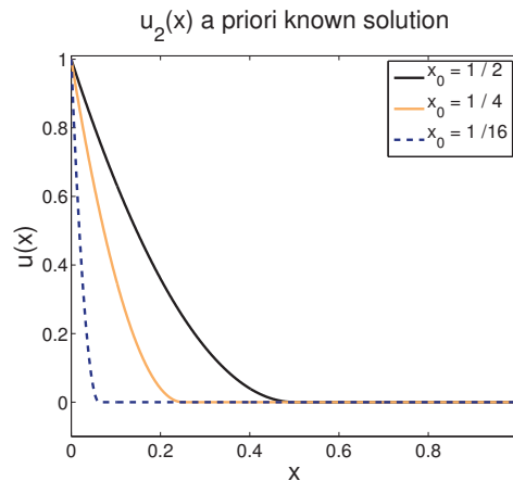
Figure 2: Representation of u_2(x) for different values of x_0 .
