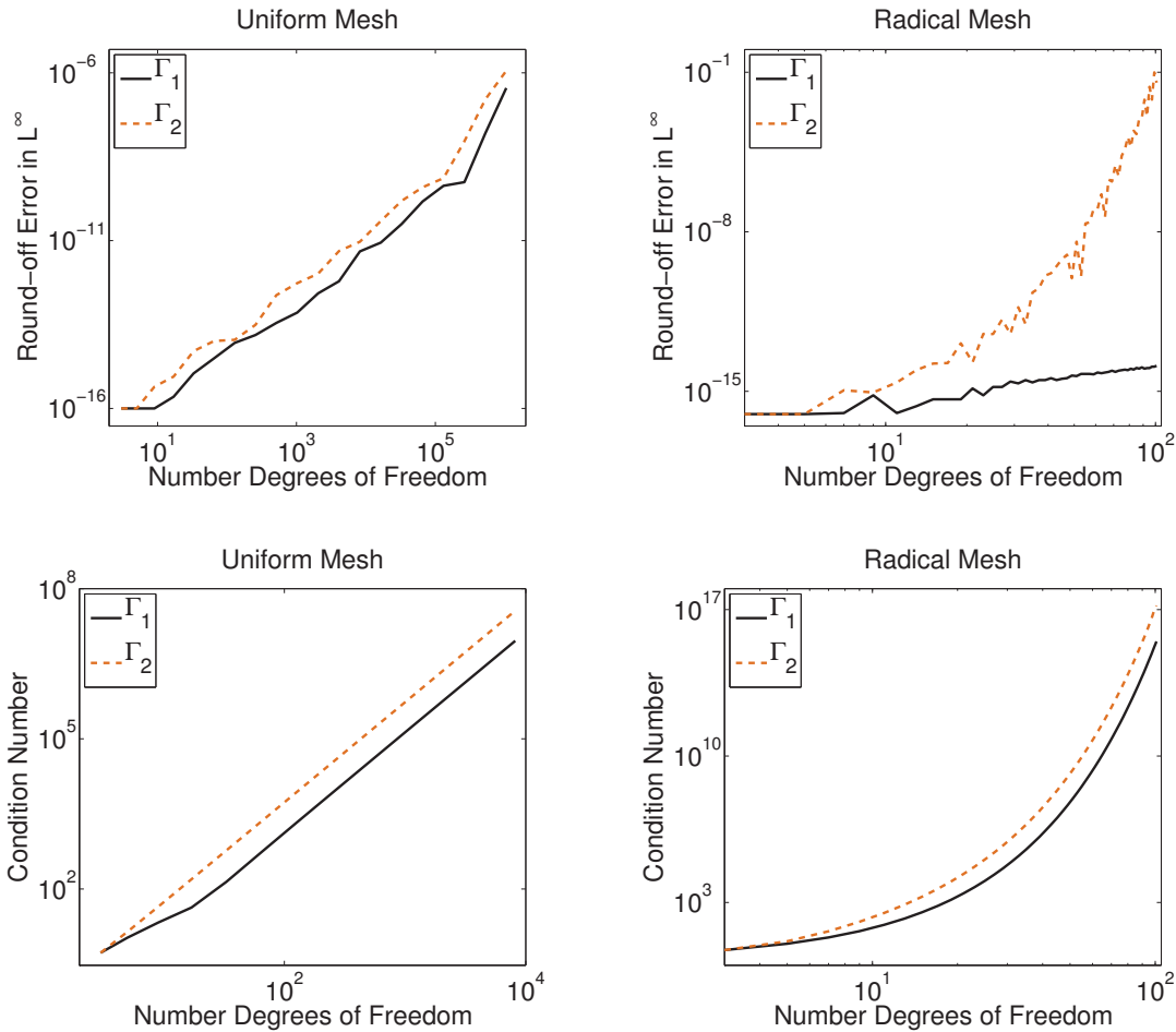
Figure 3: Log-Log representation of the condition number and round-off error for 1D Laplace problem discretized with a uniform grid (left) and a radical mesh (right). ILP shape functions of order p = 2 are used.
