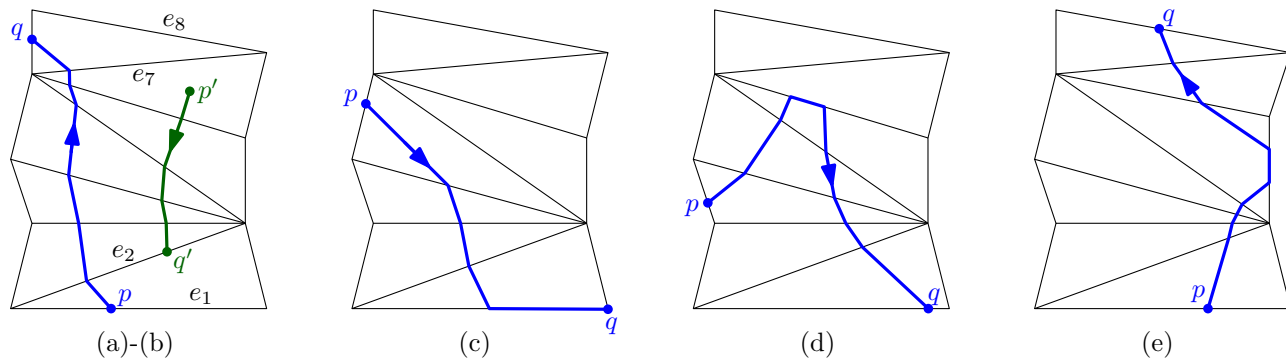
Figure 8: Shortest paths in a strip. In the first figure, the path p - q is of type (a) and the path p' - q' is of type (b).
