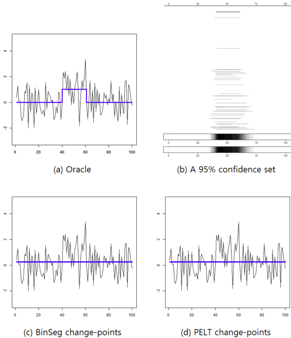
Figure 3. Plots of the simulated dataset along with horizontal lines for the underlying means in (a) and the fitted means in (c)–(d). A 95% confidence set for the cluster is in (b) with \hat{C} = \{i \mid |i - 51| \leq 10\} , \hat{\mu} = -0.008 and \hat{\theta} = 1.206 . The true cluster is C = \{i \mid |i - 50| \leq 10\} , and (\mu, \theta, \sigma^2) = (0, 1, 1) .
