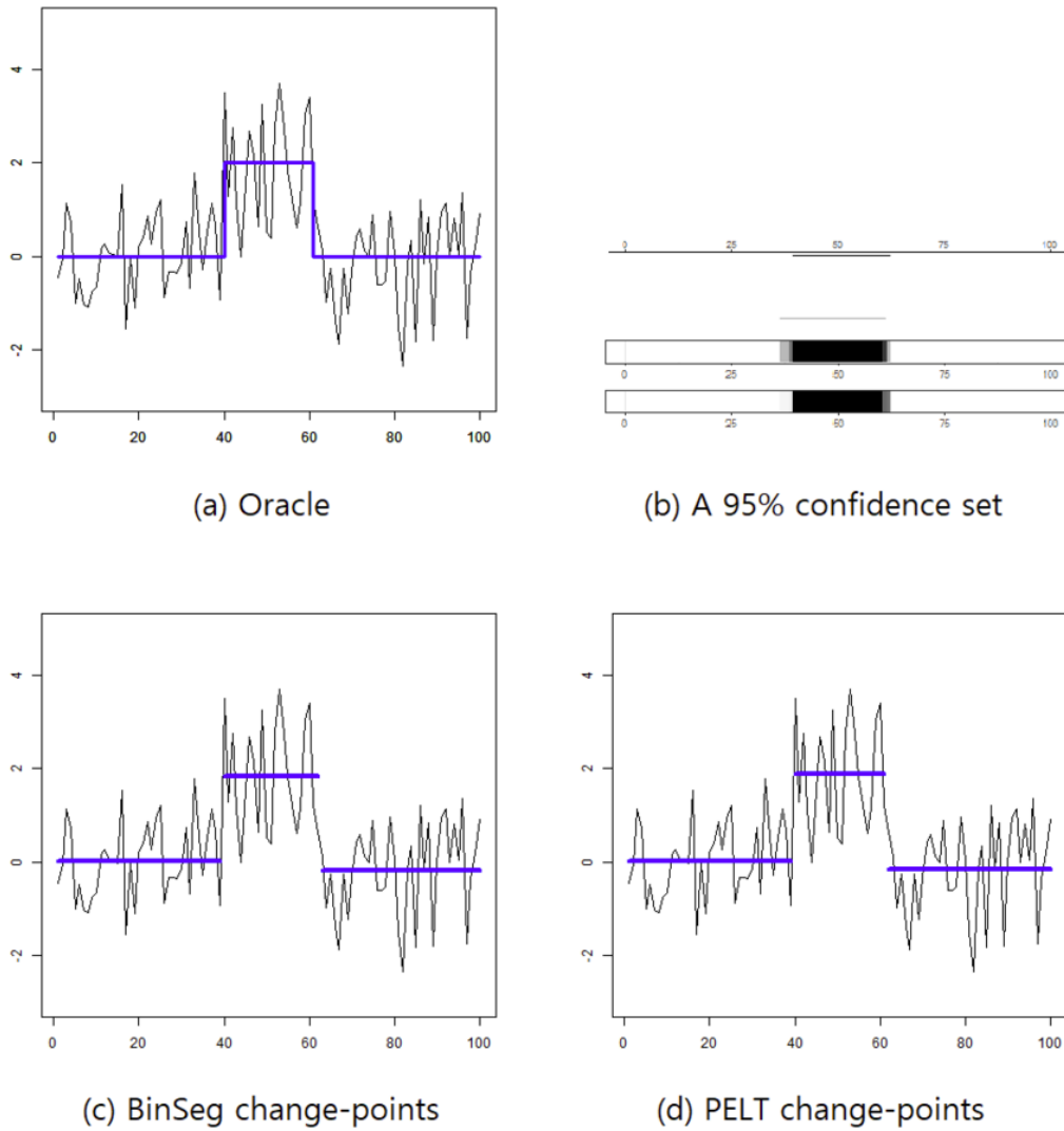
Figure 4. Plots of the simulated dataset along with horizontal lines for the underlying means in (a) and the fitted means in (c)–(d). A 95% confidence set for the cluster is in (b) with \hat{C} = \{i \mid |i - 51| \leq 11\} , \hat{\mu} = -0.081 and \hat{\theta} = 1.909 . The true cluster is C = \{i \mid |i - 50| \leq 10\} , and (\mu, \theta, \sigma^2) = (0, 2, 1) .
