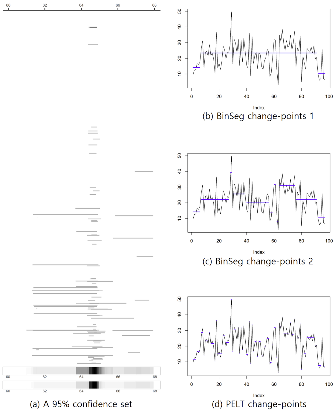
Figure 5. A 95% confidence set for the cluster is in (a) with \hat{C} = \{\text{latitude} \mid |\text{latitude} - 64.63| \leq 0.22\} , \hat{\mu} = 20.758 \text{ m}^2\text{ha}^{-1} , \hat{\theta} = 10.345 \text{ m}^2\text{ha}^{-1} and \hat{\sigma} = 8.108 \text{ m}^2\text{ha}^{-1} . Plots of y_i 's along with horizontal lines for the fitted means in (b)–(d).
