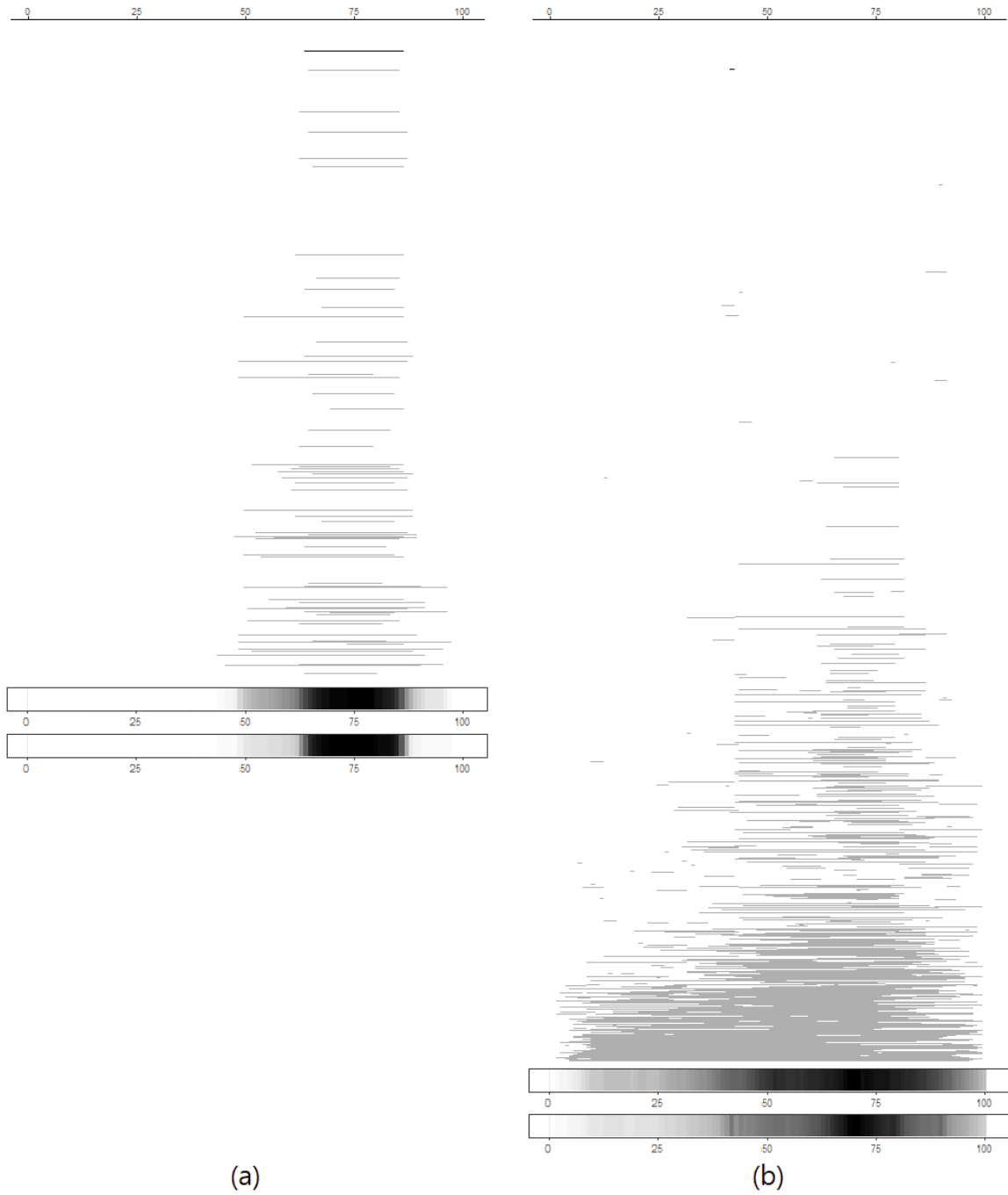
Figure 2. 95% confidence sets \Psi_{.95}(C_0) from a simulated datasets, where N = 100 , the true cluster is set to be C_0 = \{i \mid |i - 75| \leq 10\} , and signal-to-noise ratio ( \theta/\sigma ) is set to be 1 in (a) or 0.5 in (b), respectively. The set of candidate clusters \mathcal{C} is pre-defined as (9) with R_{\max} = 24 . The number of candidate clusters is |\mathcal{C}| = 2500 . The size of confidence set is |\Psi_{.95}(C_0)| = 70 in (a) and |\Psi_{.95}(C_0)| = 1613 in (b), respectively.
