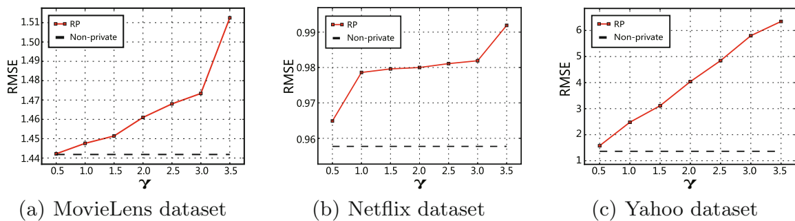
Fig. 2. RP’s effect on recommendation accuracy
