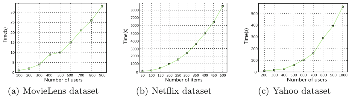
Fig. 8. Efficiency of the hybrid approach
