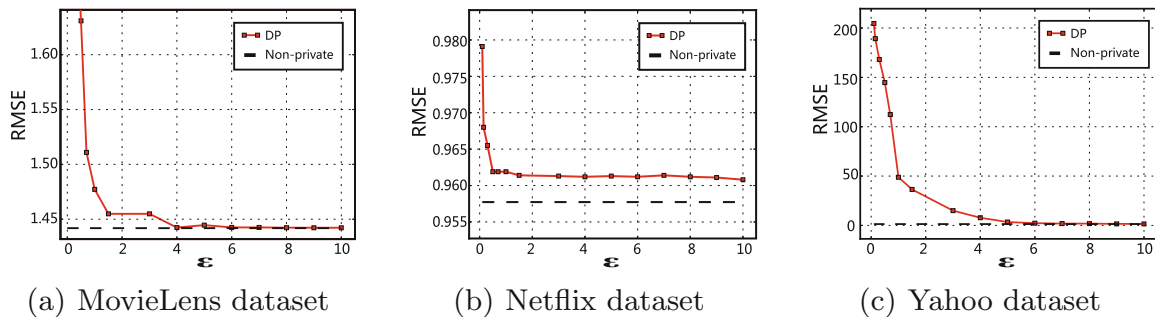
Fig. 3. DP’s effect on recommendation accuracy
