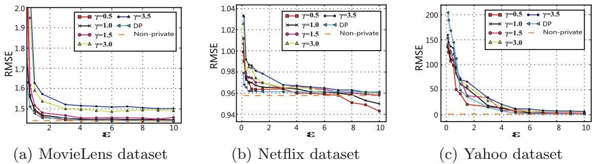
Fig. 4. RP's effect on DP
