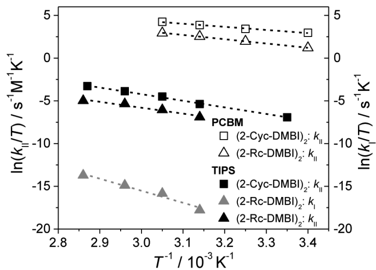
Figure 7. Eyring plots for variable-temperature rate-constant data for PCBM and TIPSp doped with (Y-DMBI) 2 derivatives.
