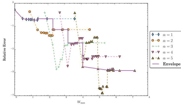
15 16 17 18 19 20 21 22 23 24 25 26 27 28 29 30 31 32 33 34 35 36 37 38 39 40 41 42 43 44 45 46 47 48 49 50 51 52 53 54 55 56 57 58 59 60 61 62 63 64 65 Figure 4: Envelope of SGSC convergence curves for the test case with d = 3 and N = 10 .
