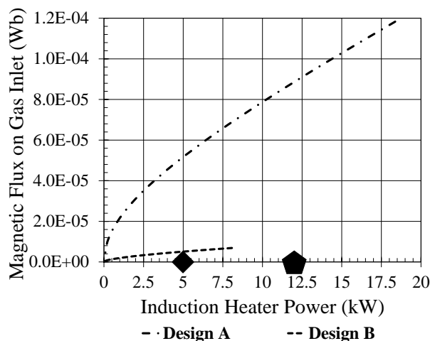
Fig. 6 The magnetic flux on the gas inlet versus the induction heater power. The pentagon and the rhombus indicate the required induction power for reaching the substrate temperature of 1600 °C in Design A and Design B, respectively.
