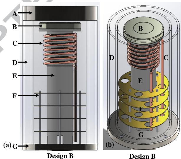
Fig. 2 (a) The side view and (b) isometric view of the proposed design (Design B) without the gas inlet, where A, B, C, D, E, F, and G represent the gas inlet, T-shaped susceptor, induction
