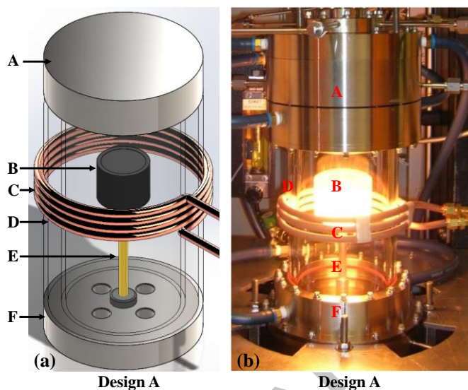
Fig. 1 (a) Isometric view of the conventional induction-heating MOCVD reactor (Design A) and (b) a photograph (courtesy of Prof. Z. Sitar, NCSU) of Design A. A, B, C, D, E, and F represent the gas inlet, susceptor, induction coil, double quartz wall, susceptor supporter, and bottom flange, respectively.
