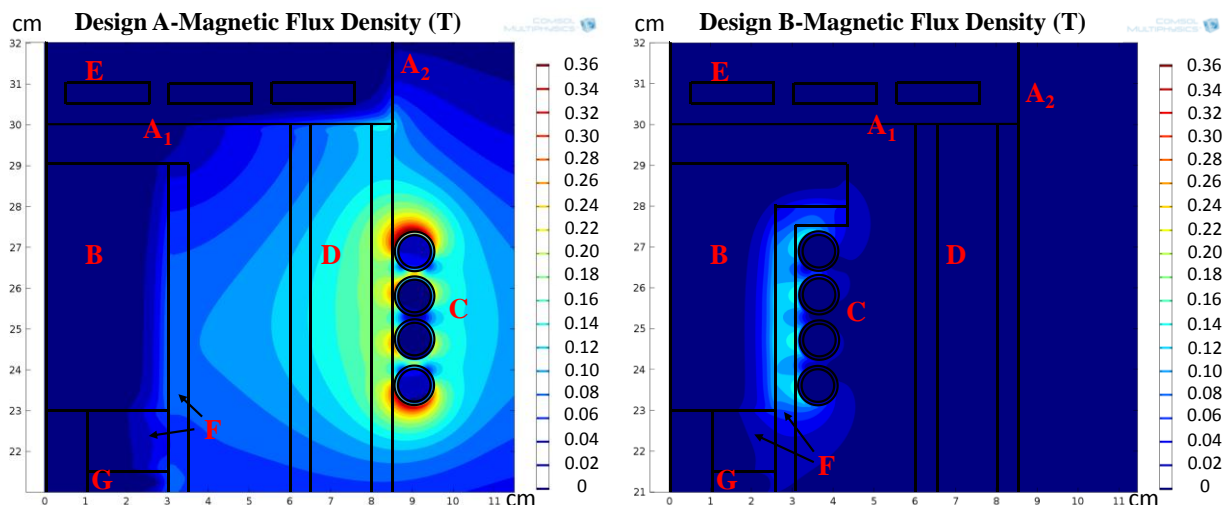
Fig. 5 Cross-sectional view of the magnetic flux density of (a) Design A and (b) Design B at 1600 °C, where B, C, D, E, F, and G represent the susceptor, induction coil, double quartz wall, cooling water channel, thermal insulator, and supporter respectively. A 1 and A 2 are the bottom surface and lateral surface of the gas inlet, respectively.
