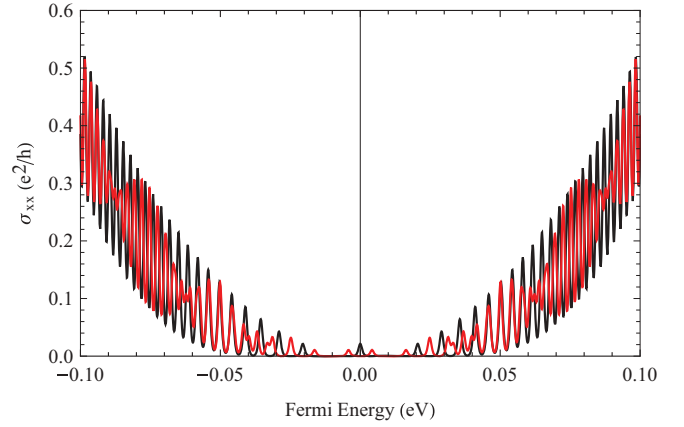
FIG. 1. (Color online) Collisional conductivity as a function of Fermi energy for zero (black lines) and finite (red lines) strain energy. The velocity is taken to be 4 \times 10^5 m/s, B = 2 T, T = 5 K, and \Delta = 4.2 meV.
