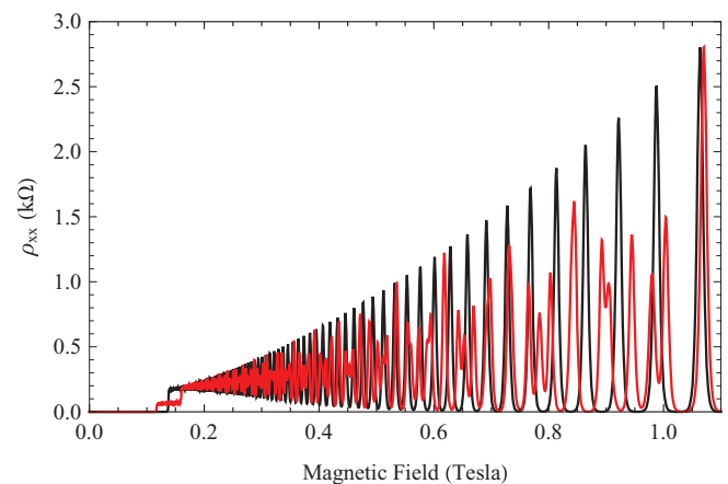
FIG. 3. (Color online) Collisional resistivity as a function of magnetic field, using the same parameters as in Fig. 2.
