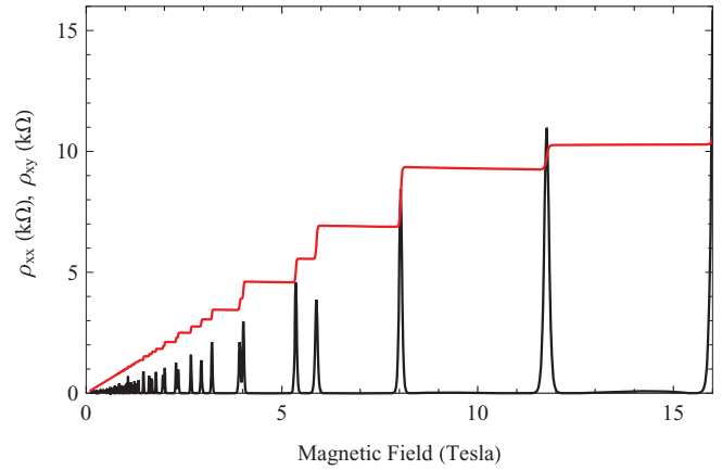
FIG. 2. (Color online) Collisional (black lines) and Hall (red lines) resistivities as a function of magnetic field for a fixed value of the strain energy. The velocity is taken to be 4 \times 10^5 m/s, the Fermi energy to be 54 meV, T = 1 K, and \Delta = 4.2 meV.
