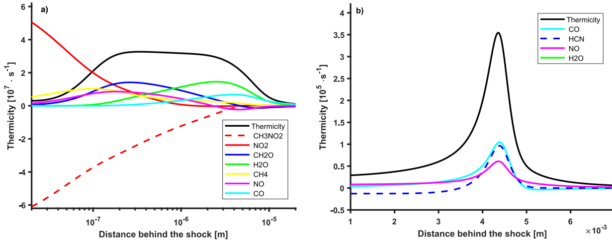
Fig. 5. Species contributing to the first (in a) and second (in b) thermicity peaks as a function of the distance behind the shock. The thermicity profiles and the species contributing to it are represented in black and colored lines, respectively. The results were obtained with Le’s model for a pure \text{CH}_3\text{NO}_2 detonation at T_1 = 383\text{K} and P_1 = 80\text{kPa} initial conditions.
