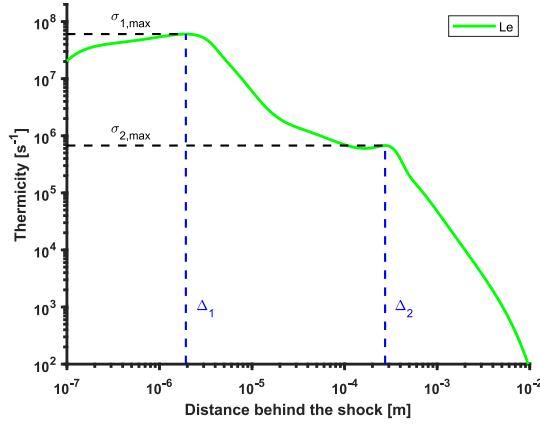
Fig. 1. Thermicity profile as a function of the distance behind the shock, obtained with Le's model with the following mixture: x_{\text{NM}} = 0.8 , x_{\text{O}_2} = 0.2 , T_1 = 383 \text{ K} , P_1 = 100 \text{ kPa} , and a Chapman-Jouguet detonation speed. The local maxima ( \sigma_1 and \sigma_2 ) are employed to determine the two induction lengths ( \Delta_{1,\text{max}} and \Delta_{2,\text{max}} ), based on their appearance orders.
