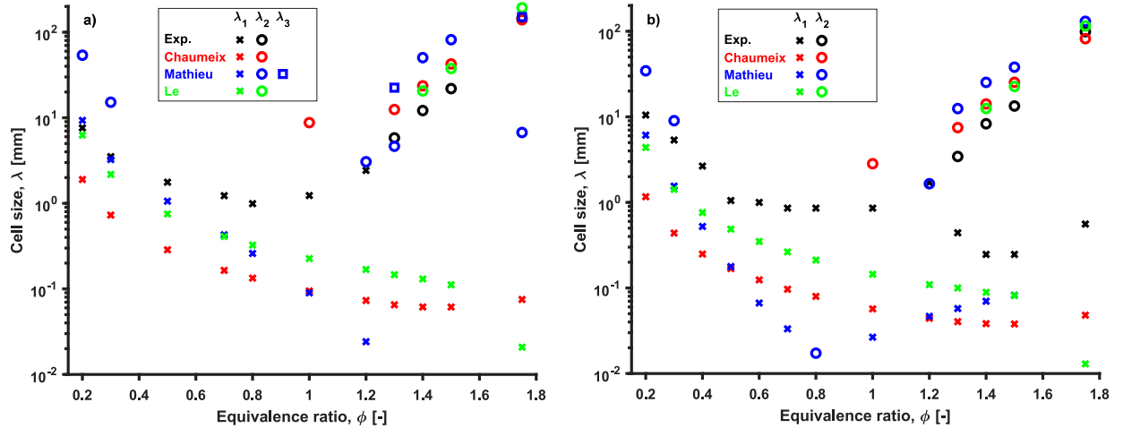
Fig. 2. Experimental (black symbols) and simulated (colored symbols) cell size evolution as a function of the equivalence ratio ( \phi ) for the validation cases 1 (in a) and 2 (in b). Chaumeix, Mathieu, and Le's reaction models are in red, blue, and green, respectively. The conditions in a are from [1]: \phi = 0.2 - 1.75 , T_1 = 390 \text{ K} , and P_1 = 50 \text{ kPa} . The conditions in b are from [2]: \phi = 0.2 - 1.75 , T_1 = 383 \text{ K} and P_1 = 80 \text{ kPa} .
