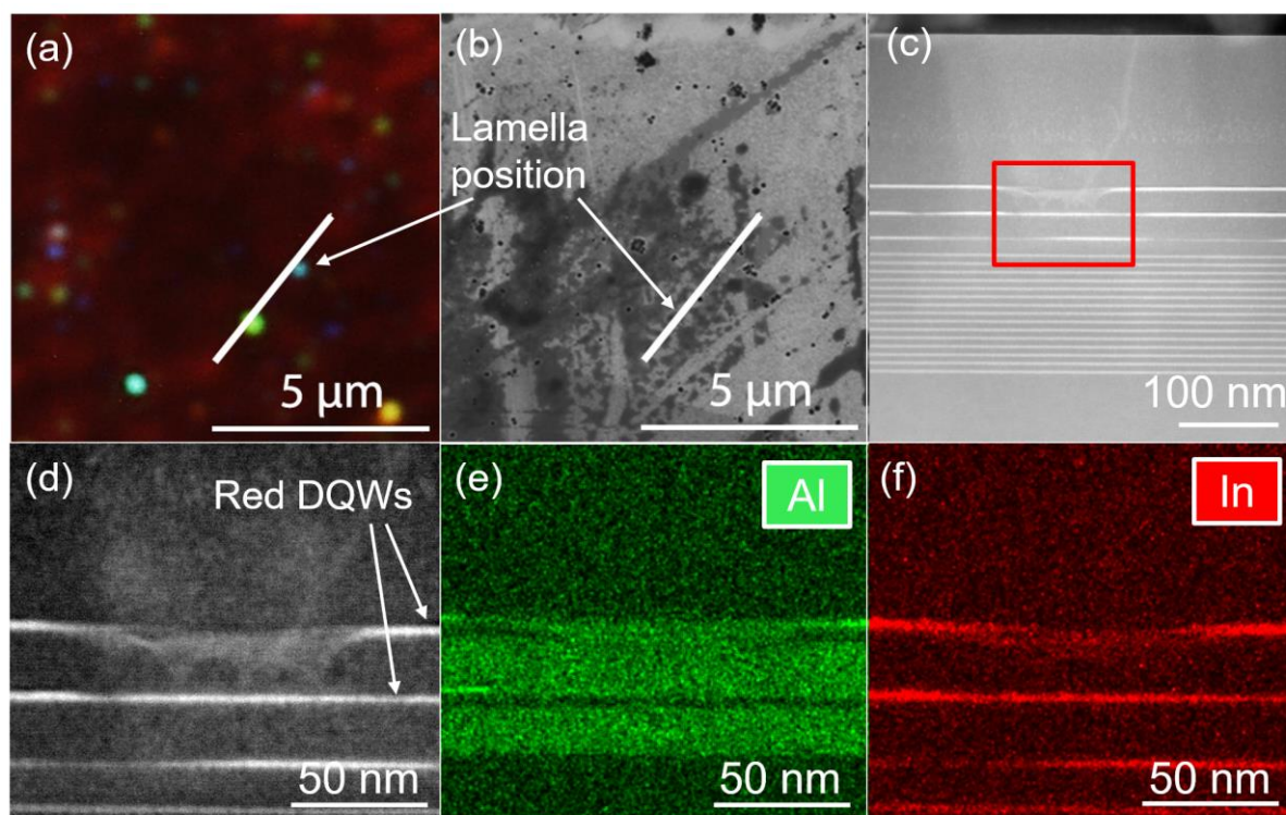
Figure 5. (a) EL mapping and (b) scanning electron microscope (SEM) image used for the lamella positioning. (c) scanning transmission electron microscope (STEM) image and (d) high-resolution STEM image of our active region structure. (e) Al and (f) In atom distribution mapping in the active region by STEM energy dispersive X-ray spectroscopy (EDS) measurements.
