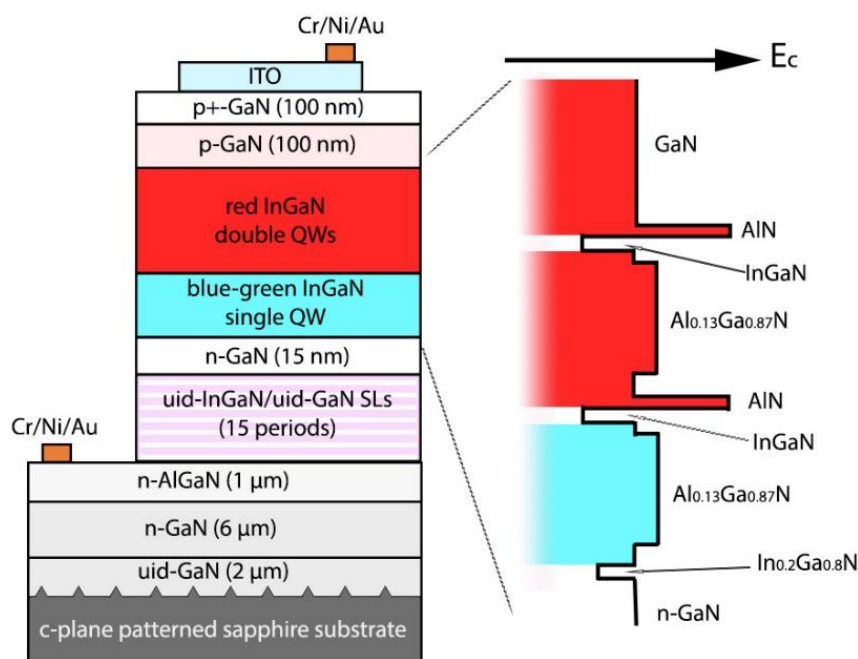
Figure 1. Red indium gallium nitride (InGaN) light-emitting diode (LED) epistructure and conduction band profile in the active region.
