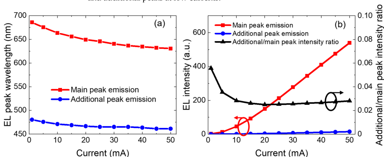
Figure 3. Current dependence of (a) the peak wavelengths (b) EL intensity and intensity ratio for additional short-wavelength and red quantum well (QW) emission.
