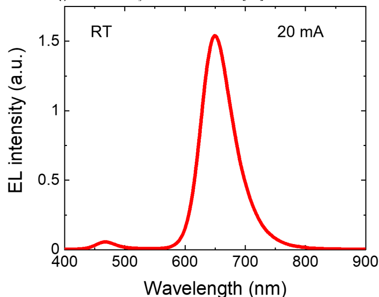
Figure 2. Electroluminescence (EL) spectrum of the red LED at 20 mA.
