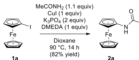
Scheme 1. N -arylation of acetamide with iodoferrrocene.
