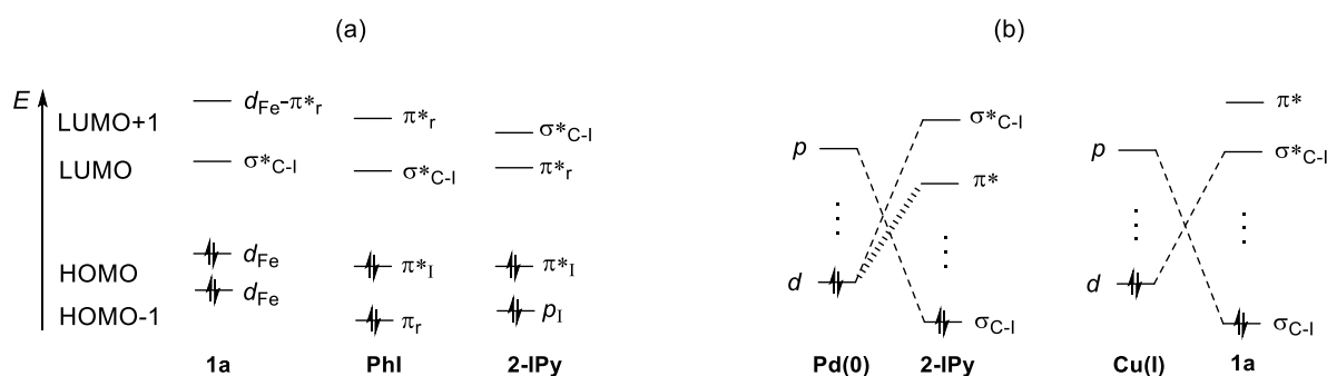
Scheme 2. (a) FMO profile of the selected species; (b) schematic representation of the allowed interactions between 2-iodopyridine ( 2-IPy ) and Pd(0) [24] vs those of iodoferrocene ( 1a ) and Cu(I).
