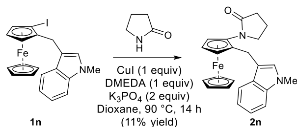
Scheme 3. Reaction from 1n .
