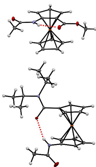
Figure 3. Hydrogen bonds observed at the solid state for compounds 2i (top) and 6j (bottom). Thermal ellipsoids shown at the 30% probability level. Cp-Cp planes angles 0.5(0.2) and 4.0(0.2) ° for 2i and 6j , respectively.
