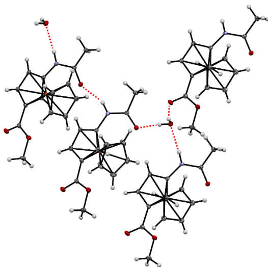
Figure 2. Hydrogen bonds network observed at the solid state for compound 4i . Thermal ellipsoids shown at the 30% probability level. Cp-Cp planes angles 2.3(0.3) and 3.6(0.3) °.
