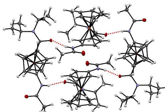
Figure 4. Hydrogen bonds observed at the solid state for compounds 4j . Thermal ellipsoids shown at the 30% probability level.
