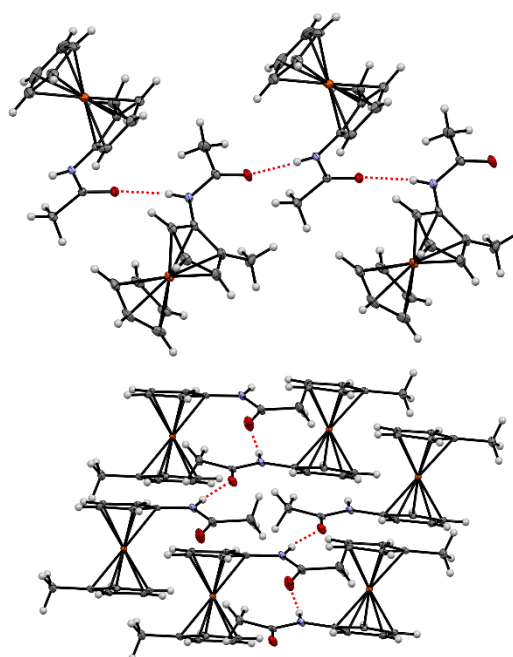
Figure 1. Hydrogen bonds network observed at the solid state for compounds 2b (top) and 6b (bottom). Thermal ellipsoids shown at the 30% probability level. Cp-Cp planes angles (3.4(0.3) and 0.6(0.3) °) and (0.4(0.3) and 0.6(0.3) °) for 2b and 6b , respectively.
