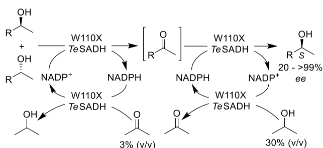
Scheme 1. Scheme 1. One-pot two-step deracemization of alcohols using a single TeSADH mutant. X = G or A. R = Phenyl-ring-containing substituents.
