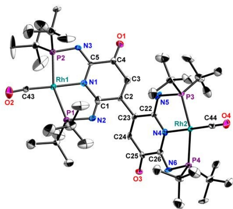
Figure 2. Molecular structures of 3 . Thermal ellipsoids are shown at the 50% probability level. Selected bond length [Å] and bond angles [°]: C4-O1, 1.23(2); C2-C3, 1.30(3); C43-O2, 1.147(19); C5-N3, 1.28(2); C1-N2, 1.28(2); Rh1-N1, 2.040(13); Rh1-C43, 1.834(16); Rh1-P1, 2.289(5); Rh1-P2, 2.292(5); C2-C23, 1.49(2); C25-O3, 1.23(2); C23-C24, 1.35(3); C44-O4, 1.17(2); C26-N6, 1.32(2); C22-N5, 1.28(2); Rh2-N4, 2.054(12); Rh2-C44, 1.82(2); Rh2-P3, 2.278(11); Rh2-P4, 2.276(5); N1-Rh1-C43, 178.3(7); P1-Rh1-P2, 159.05(17); N1-Rh1-P1, 79.8(4); P1-Rh1-C43, 101.5(6); C43-Rh1-P2, 99.4(6); P2-Rh1-N1, 79.3(4); N4-Rh2-C44, 178.2(7); P3-Rh2-P4, 160.3(3); N4-Rh2-P3, 80.8(5); P3-Rh2-C44, 98.5(6); C44-Rh2-P4, 100.7(6); P4-Rh2-N4, 79.9(4).
