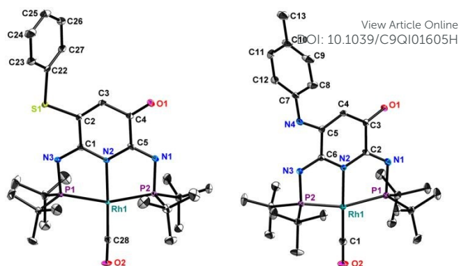
Figure 3. Molecular structures of 5 (left) and 6 (right). Thermal ellipsoids are shown at the 50% probability level; hydrogen atoms are omitted for clarity. Selected bond length [Å] and bond angles [°]: for 5 : C4-O1, 1.220(3); C2-C3, 1.346(4); C2-S1, 1.753(3); C28-O2, 1.151(4); C1-N3, 1.295(4); C5-N1, 1.294(4); Rh1-N2, 2.061(2); Rh1-P1, 2.2849(7); Rh1-C28, 1.824(3); Rh1-P2, 2.2978(7); N2-Rh1-C28, 177.65(10); P1-Rh1-P2, 159.49(2); N2-Rh1-P1, 80.19(6); P1-Rh1-C28, 98.42(8); C28-Rh1-P2, 101.94(8); P2-Rh1-N2, 79.38(6). For 6 : C3-O1, 1.235(6); C4-C5, 1.362(7); C5-N4, 1.351(7); C1-O2, 1.156(7); C6-N3, 1.295(7); C2-N1, 1.291(8); Rh1-N2, 2.049(4); Rh1-C1, 1.810(6); Rh1-P2, 2.3054(15); Rh1-P1, 2.2894(15); N2-Rh1-C1, 179.0(3); P2-Rh1-P1, 158.56(6); N2-Rh1-P2, 79.85(13); P2-Rh1-C1, 100.85(19); C1-Rh1-P1, 99.78(19); P1-Rh1-N2, 79.46(13).
