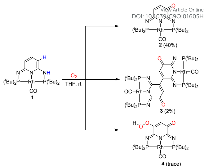
Scheme 3. Reaction of 1 with O_2 at room temperature.
