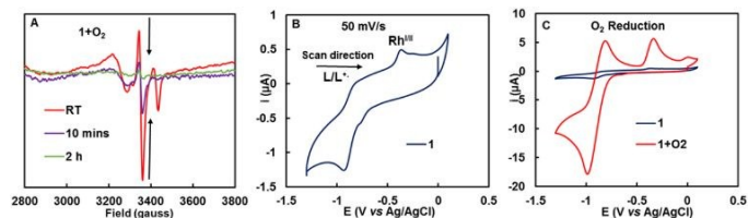
Figure 4. A) Detection of reaction intermediate in the reaction between 1 and O 2 with EPR spectroscopy. Conditions: T = 10 K, freq. = 9.3931 GHz, att. = 20 dB. B) Cyclic voltammogram of 1 in THF (1.0 mM of complex 1 , scan rate: 50 mV/s, Glassy carbon electrode (GC, diameter 3 mm) as a working electrode, Pt-wire as a counter electrode, Ag/AgCl/1M KCl as a reference electrode, 0.1 M n Bu 4 NPF 6 as a supporting electrolyte. C) Electrochemical investigation of 1 in presence of O 2 , with clear indication of reduction current (enhancement of current) (scan rate: 50 mV/s).
