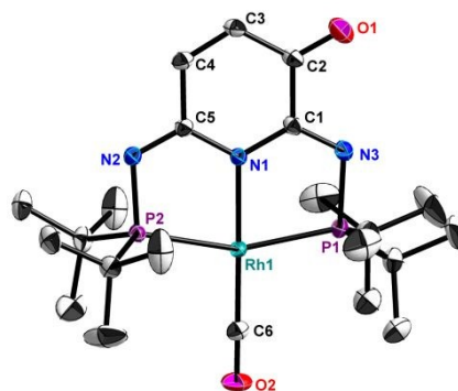
Figure 1. Molecular structures of 2 . Thermal ellipsoids are shown at the 50% probability level. Selected bond length [Å] and bond angles [°]: C2-O1, 1.233(4); C3-C4, 1.358(4); C6-O2, 1.150(4); C1-N3, 1.285(3); C5-N2, 1.291(3); Rh1-N1, 2.059(2); Rh1-C6, 1.824(3); Rh1-P1, 2.2921(6); Rh1-P2, 2.2918(7); P2-Rh1-P1, 159.33(2); N1-Rh1-C6, 178.65(13); P2-Rh1-N1, 79.70(6); N1-Rh1-P1, 79.63(6); P2-Rh1-C6, 100.76(10); C6-Rh1-P1, 99.91(10).
