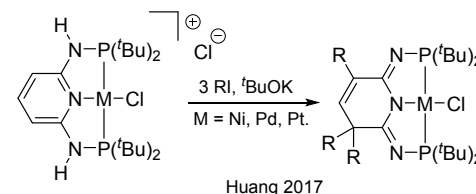
Scheme 1. Various reactivities in pincer metal complexes.
