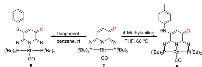
Scheme 4. Oxidative Michael addition of 2 .
