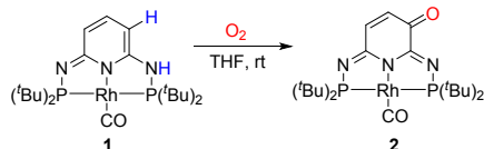
Scheme 2 Reactions between organometallic complex and O_2 .
