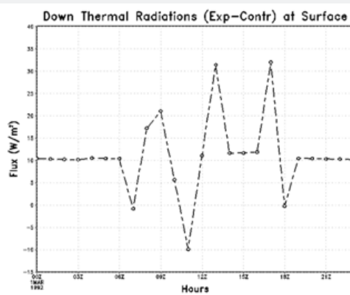
Figure 7: Change in the mean downward thermal radiation's diurnal cycle at the surface based on doubled CO 2 forcing (Experiment-Control).
