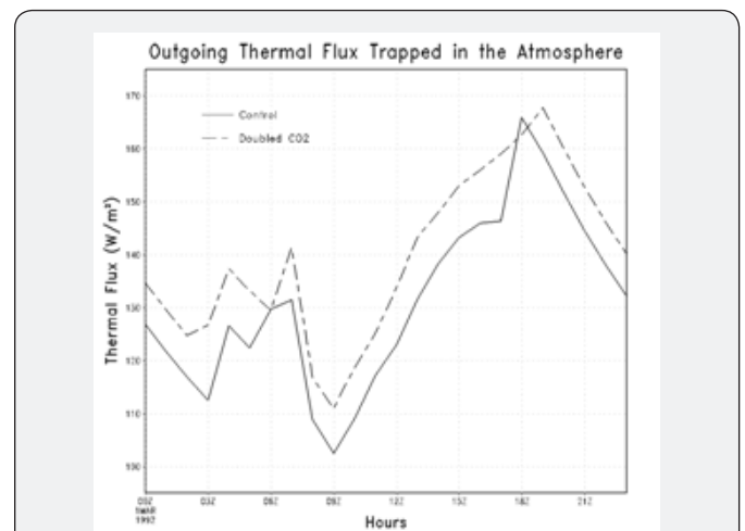
Figure 4: Mean diurnal pattern of outgoing thermal radiation's trapped between the surface and outermost layer of the troposphere.
