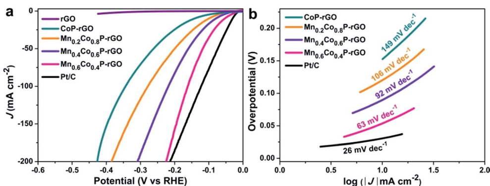
Fig. 4 Electrocatalytic HER performance of \text{Mn}_x\text{Co}_{1-x}\text{P-rGO} ( x = 0.6, 0.4, 0.2, 0 ) loaded on carbon paper in 1 M KOH: (a) IR-corrected polarization curves of the \text{Mn}_x\text{Co}_{1-x}\text{P-rGO} , rGO, and 20 wt% Pt/C. (b) The corresponding Tafel plots.
