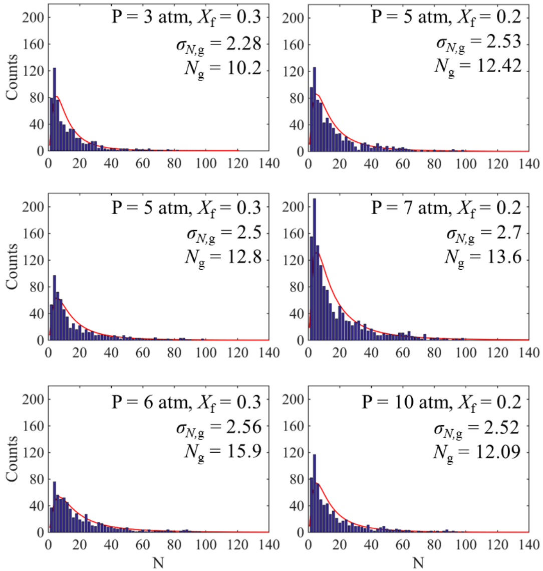
Fig. 2S. Aggregate size distribution in pressurized flames
