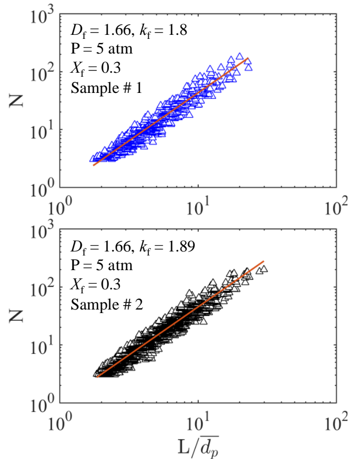
Fig.1S. Log-log plot of N vs L/\overline{d}_p for aggregates analyzed from different samples at similar operating conditions
