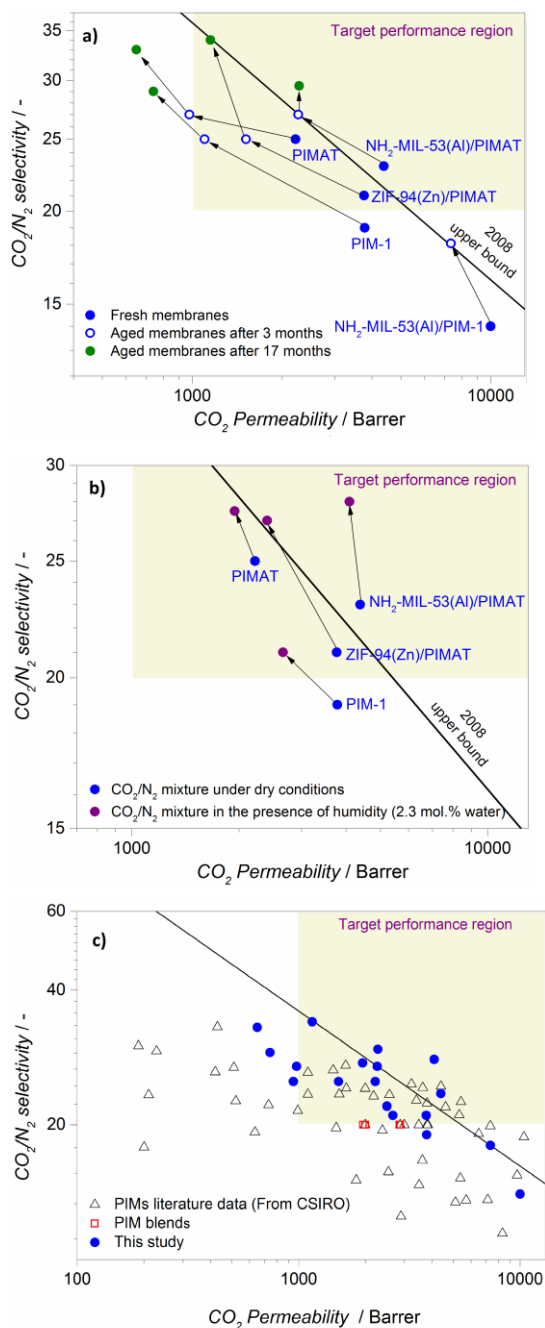
Figure 3. a) Robeson plot of \text{CO}_2/\text{N}_2 separation performance of the fresh (blue closed), aged membranes after 3 months (blue open symbols) and 17 months (green closed squares) tested under dry conditions. b) Robeson plot of \text{CO}_2/\text{N}_2 separation performance of the fresh (blue symbols) membranes tested under dry and humid (2.3 mol.% water in feed, purple symbols) conditions. c) Robeson plot of \text{CO}_2/\text{N}_2 mixed gas separation performance of this study (the fresh/aged membranes in dry and humid condition) and the literature data of microporous polymers taken from Commonwealth Scientific and Industrial Research Organization (CSIRO). [27] The Robeson upper bound (2008) [2] is shown for reference, as well as the target performance region for \text{CO}_2 capture from flue gas from Merkel et al. [16] assuming a membrane thickness of 1 \mu\text{m} . The MOF particle loading in PIMAT is 25 wt.%. The Matrimid® loading in PIM-1 is 9.1 wt.%. All the measurements were conducted at 298 K with 2 bar absolute feed pressure (mixed gases). 1 Barrer = 1 \times 10^{-10} \text{ cm}^3 \text{ (STP) cm cm}^{-2} \text{ s}^{-1} \text{ cmHg}^{-1} .
