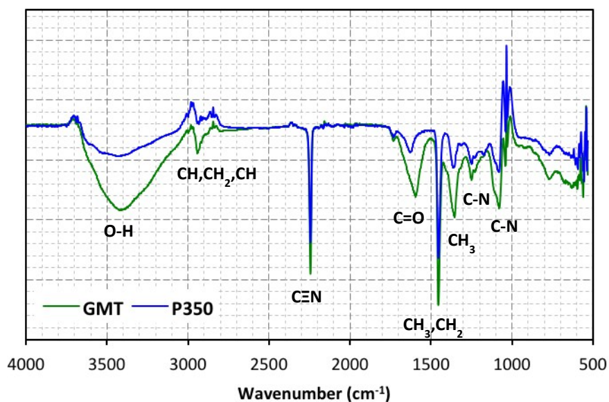
Fig. S4 ATR-IR of GMT and P350 Support
