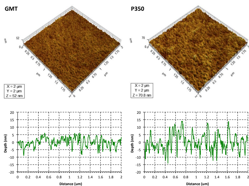
Fig. S5 AFM images of the supports.
