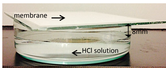
Fig. S3 Cellulose regeneration using acid vapor
