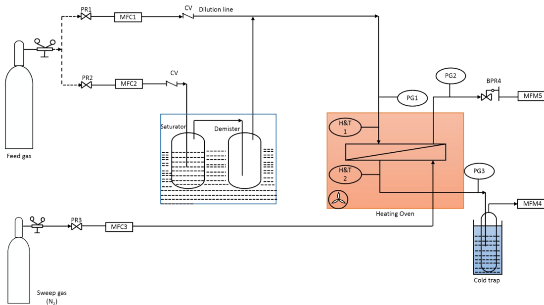
Fig. S2 Dehumidification experimental setup.
