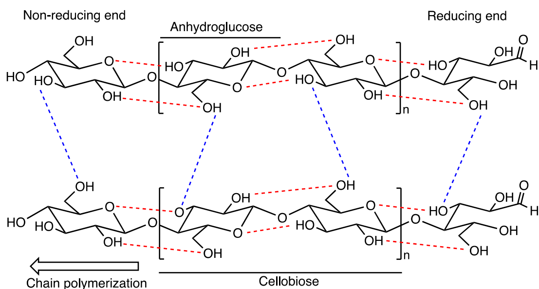
Fig. S1 Cellulose structure with the intra- and inter-chain hydrogen bonds.
