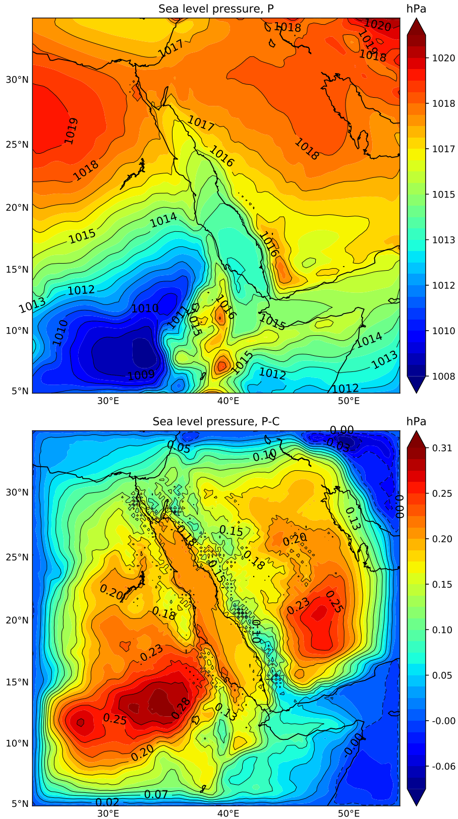
Figure S1. January climatology of the sea level pressure. Top panel shows the WRF P mean state and bottom panel shows the WRF P-C anomaly due to dust.
