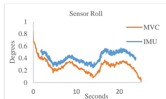
Figure 7 – Data from a single pass comparing the roll measured by the IMU and the roll as calculated from the MVC camera data.
