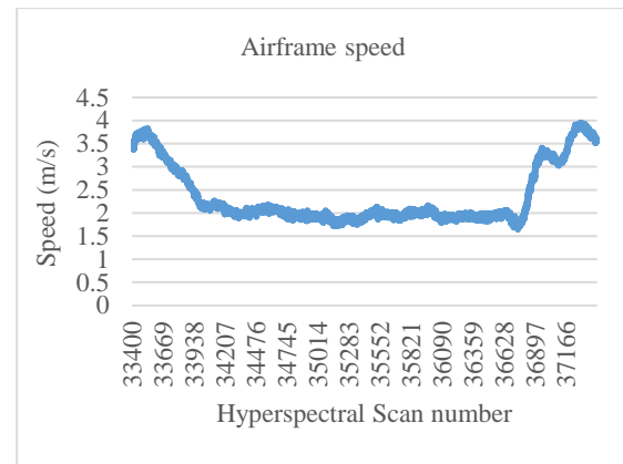
Figure 4 – Airframe speed plotted for a one pass, allowing stable section of flight to be selected.
