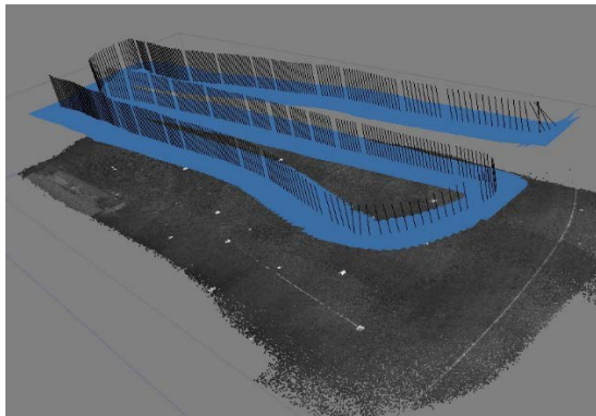
Figure 5 – Screenshot for Photoscan showing the alignment of 3 passes of image data and the sparse pointcloud that was created.
