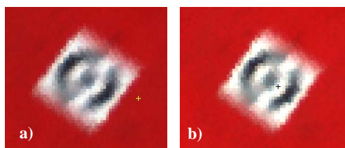
Figure 8 – a) Positional error of GCP before boresight correction and b) Error after boresight correction applied
