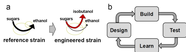
Fig. 2 Development of a cell factory. a A reference strain, e.g., a strain that can efficiently convert sugars to ethanol, is engineered by first reconstruction of a novel pathway that leads to the product of interest, here illustrated as a red pathway towards isobutanol. Thereafter, the cell factory is engineered such that the majority of the sugar is converted to the desired product and no (or little) sugar is converted to ethanol (the original product). The last step is to ensure that the engineered strain has the right titer, rate, and yield (TRY) metrics to allow for cost-competitive production of chemical. b In order to reach the TRY targets for industrial implementation, it is generally necessary to perform extensive engineering of the cell factory. This involves several rounds of the so-called Design-Build-Test (DBT) cycle. Here designs are developed based on physiological knowledge or through mathematical modeling and these designs are being built into the strain. The engineered strain(s) are then tested, preferentially at industrial-like conditions. By going through the DBT cycle, much knowledge is gained about the physiology of the cell factory, and it is important to accumulate this knowledge and learn from each design step
