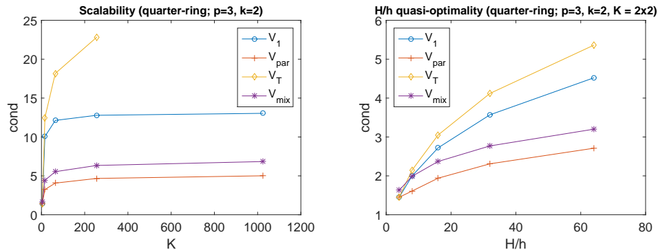
FIG. 2. Performance summary of BDDC deluxe preconditioner with minimal primal spaces V_1 ( \circ ), V_{par} ( + ), V_T ( \diamond ), and V_{mix} ( * ). Scalability plot (left): Condition number (cond) as a function of the number of subdomains K . Quasi-optimality plot (right): Condition number (cond) as a function of the ratio H/h . Quarter-ring domain, p = 3 , and k = 2 .
