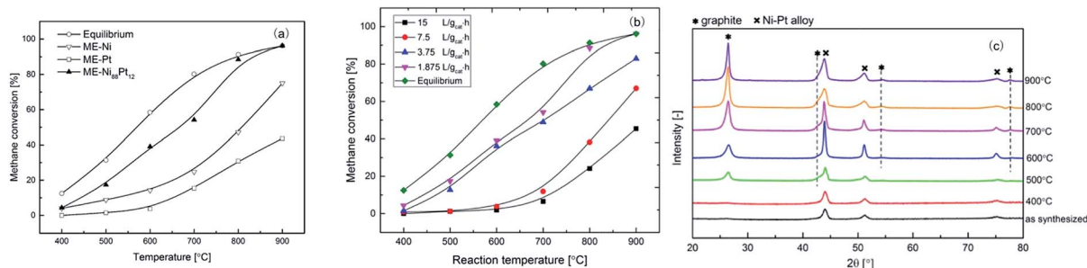
Fig. 2 (a) Activity comparison over microemulsion prepared samples at \text{SV} = 1.875 \text{ L g}_{\text{cat}}^{-1} \text{h}^{-1} ; (b) the activity of \text{Ni}_{88}\text{Pt}_{12} for methane cracking; (c) in situ XRD pattern on \text{Ni}_{88}\text{Pt}_{12} during methane cracking at 400–900 ^{\circ}\text{C} under \text{SV} = 1.875 \text{ L g}_{\text{cat}}^{-1} \text{h}^{-1} .
