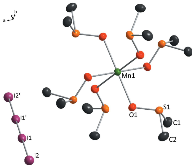
Figure 1 The molecular components of the title compound, with displacement ellipsoids drawn at the 50% probability level. H atoms have been omitted for clarity. [Symmetry code: (') \frac{4}{3} - x, \frac{2}{3} - y, \frac{5}{3} - z ]
