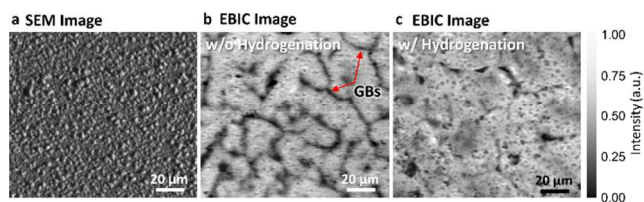
Figure 3. (a) SEM top view image of a TF-VLS InP solar cell. (b), (c) Top view EBIC images of TF-VLS InP solar cells without and with hydrogenation. The charge carrier collection is visualized by the EBIC maps. Bright areas indicate higher collection efficiency of minority carriers. Grain boundaries are visible as dark lines.
