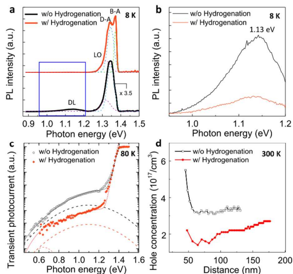
Figure 2. (a) PL spectra of TF-VLS:Zn InP ( 488 \text{ nm} Ar ion laser excitation) at 8 \text{ K} before and after hydrogenation. The fitted curves (dotted lines) are produced by using multiple-peak Gaussian fitting. (b) Enlargement of the broad DL peak seen in (a). (c) TPI spectra of TF-VLS InP solar cells with and without hydrogenation measured at 80 \text{ K} under reverse bias of -0.5 \text{ V} with filling pulse of 0.2 \text{ V} . The solid lines represent fits with the integrated sum of two Gaussian defect bands
