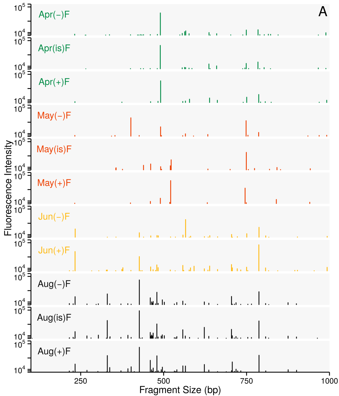
Fig. S3. Distribution of OTUs detected by ARISA for a reduced number of samples in the filtered (A) and community (B) treatments.
