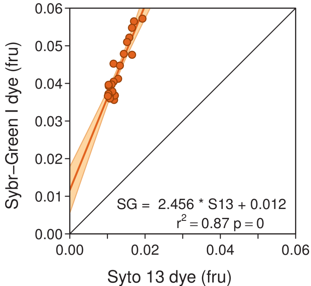
Fig. S1. Empirical calibration used to transform nucleic acid fluorescence in samples stained with Syto 13 to Sybr-Green I values in order to compare the 2002-2012 decadal mean and the 2012 experimental values shown in Fig. 1.
