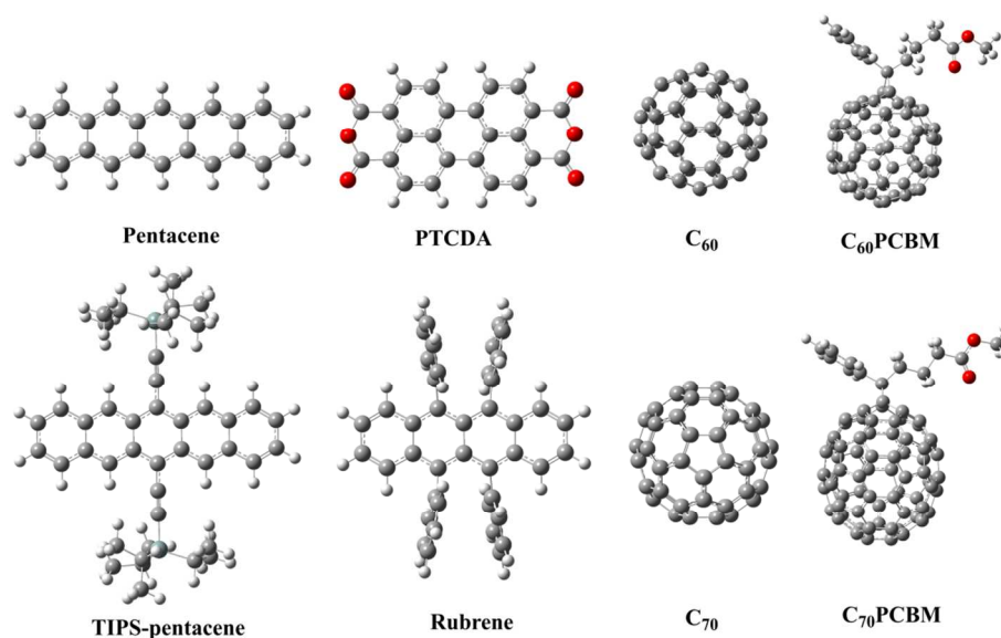
Figure 1. Molecular structures of pentacene, TIPS-pentacene, rubrene, PTCDA, C 60 , C 70 , C 60 PCBM and C 70 PCBM. The grey, white, and red atoms represent carbon, hydrogen, and oxygen, respectively.
