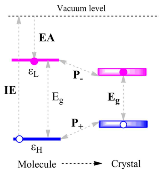
Figure 2. Schematic energy diagram of quasi-hole (electron) from gas-phase molecule to solid-state crystal; IE: ionization energy; EA: electron affinity; \epsilon_H : HOMO energy; \epsilon_L : LUMO energy; E_g : transport gap; P_+/P_- : polarization energy for hole/electron.
