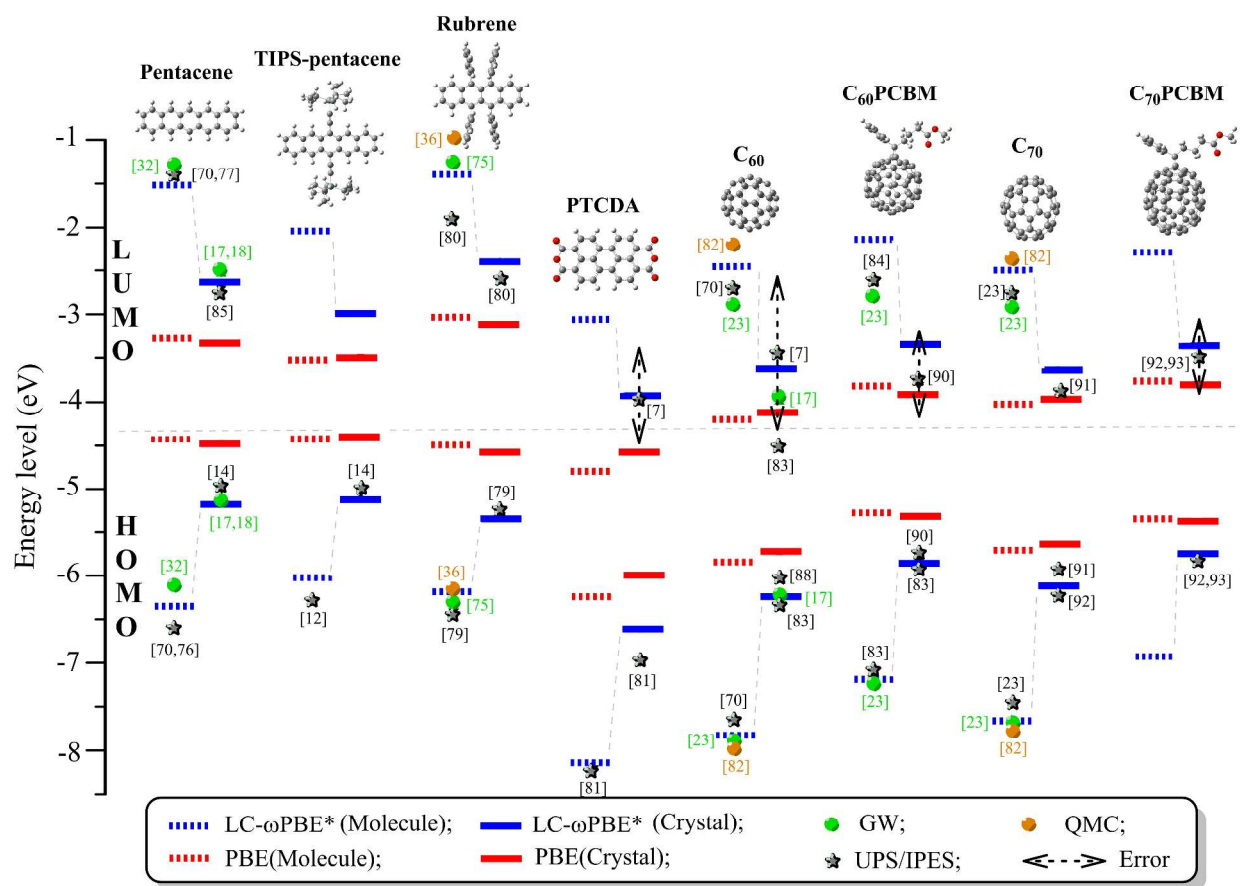
Figure 3. Calculated HOMO and LUMO energy levels from gas-phase molecules to solid-state crystals using the PBE (red) and LC- \omega PBE* (blue) functionals; the benchmarks from (self-consistent) GW, quantum Monte Carlo (QMC), and experimental data are also presented when available.
