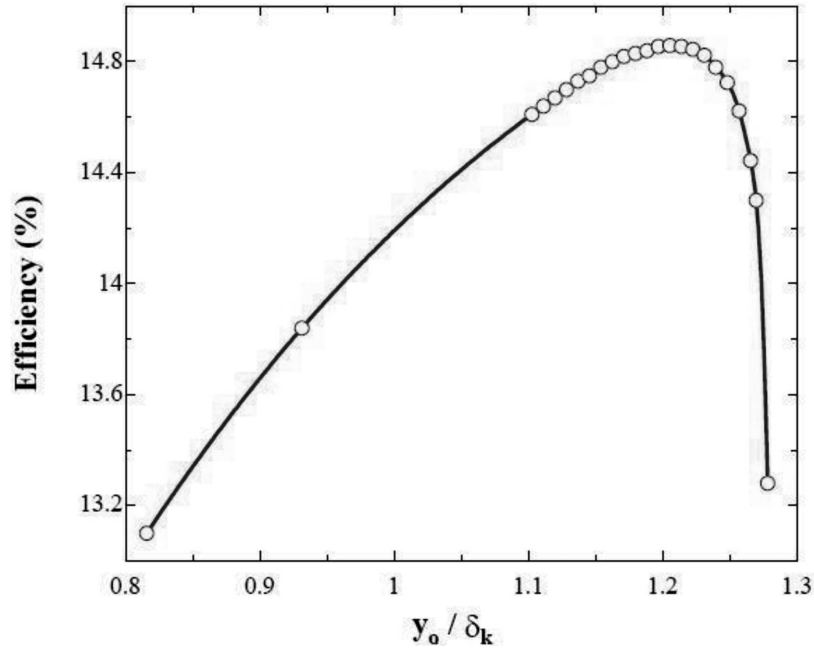
Fig. 6. Efficiency against normalized spacing of the stack plates at a constant thermal input of 2000 W to the hot heat exchanger, a frequency of 398 Hz, temperature difference of 340 K and mean helium pressure of 10 bars
