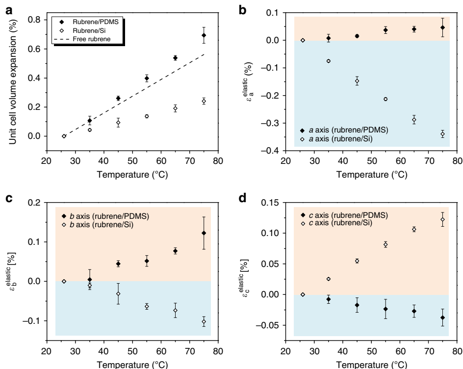
Figure 3 | Unit cell volume expansion and substrate-induced elastic mechanical strain. (a) The unit cell volume expansion for rubrene crystals laminated on PDMS and Si as a function of temperature, which are compared with that expected for free crystals. The error bars in unit cell volume expansion were based on the propagation of s.d. errors in \epsilon^{\text{total}} of the three axes as shown in Fig. 2a,b. (b) Average induced mechanical strain ( \epsilon^{\text{elastic}} = \epsilon^{\text{total}} - \epsilon^{\text{thermal}} ) along rubrene a axis as a function of temperature for crystals laminated on PDMS and Si, respectively. (c) Average \epsilon^{\text{elastic}} along rubrene b axis as a function of temperature for crystals laminated on PDMS and Si, respectively. (d) Average \epsilon^{\text{elastic}} along rubrene c axis as a function of temperature for crystals laminated on PDMS and Si, respectively. The error bars in \epsilon^{\text{elastic}} were based on the standard deviation errors in \epsilon^{\text{total}} as shown in Fig. 2a,b.
