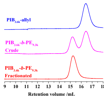
Figure 4. Monitoring the synthesis of PIB 3.6k - b -PE 9.3k by HT-GPC in 1,2,4-trichlorobenzene at 150 °C. All peaks are negative but shown in positive style for better presentation
