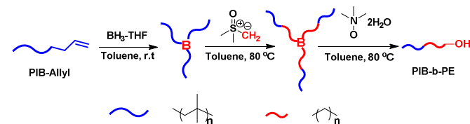
Scheme 1. General reactions for the synthesis of PIB- b -PE-OH by combining living cationic polymerization and polyhomologation
