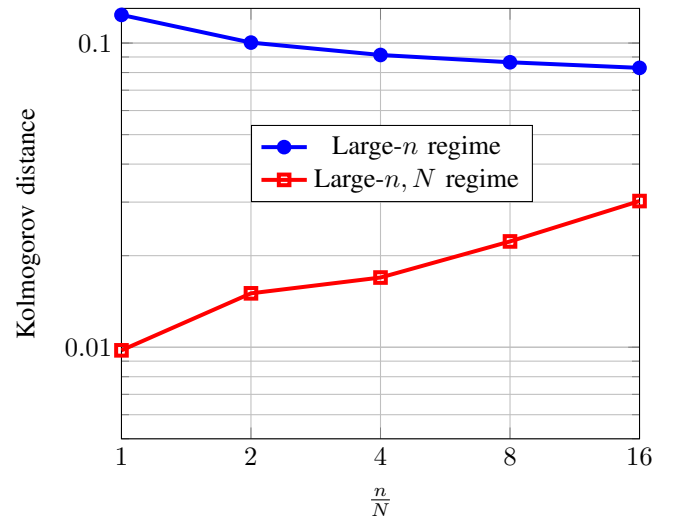
Fig. 7. Analysis of the accuracy of the CLT results for N = 32
