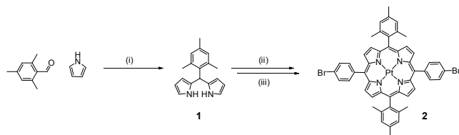
Scheme 1: Synthesis of the porphyrin precursor, (i) \text{MgBr}_2 , TFA, DCM, 50%; (ii) a) DCM, TFA, b) DDQ, 11%; (iii) PhCN, \text{PtCl}_2 , reflux, 24%
