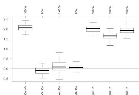
Cluster 22 / 66 genes
