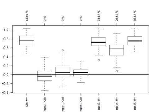
Cluster 28 / 146 genes
