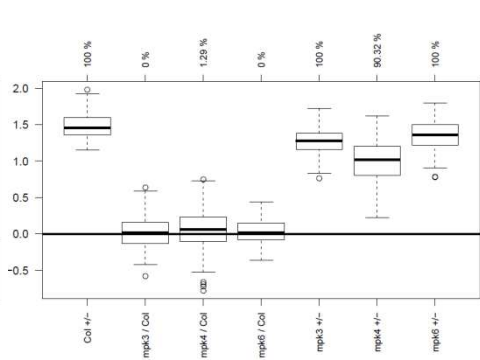
Cluster 29 / 153 genes
