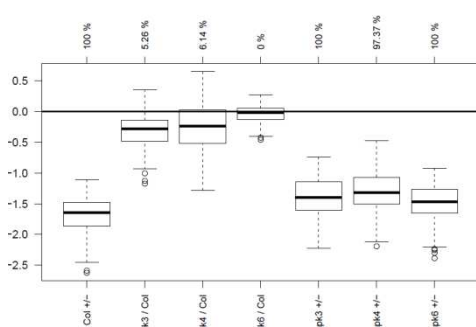
Cluster 19 / 109 genes
