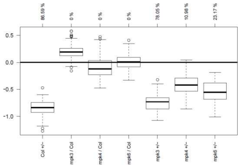
Cluster 25 / 81 genes
