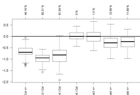
Cluster 16 / 74 genes
