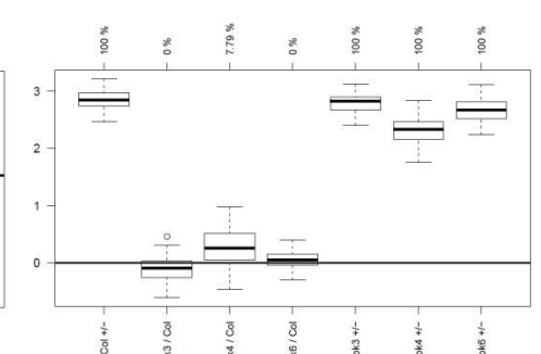
Cluster 18 / 74 genes
