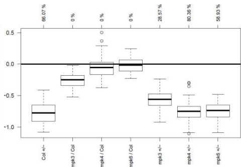
Cluster 26 / 56 genes
