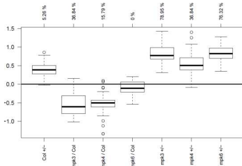
Cluster 13 / 38 genes
