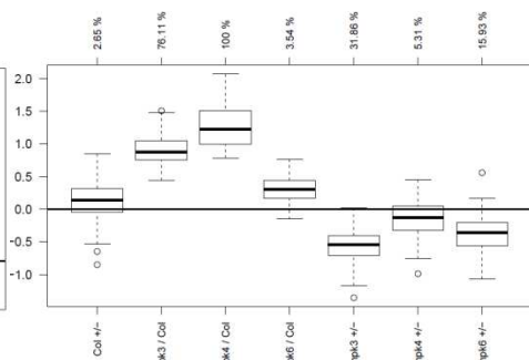
Cluster 23 / 111 genes
