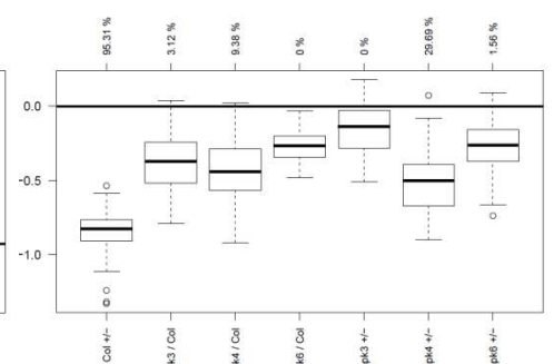
Cluster 21 / 63 genes
