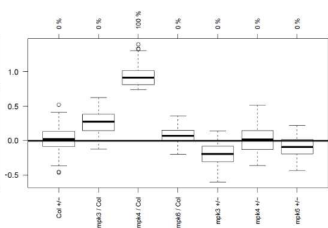
Cluster 27 / 162 genes
