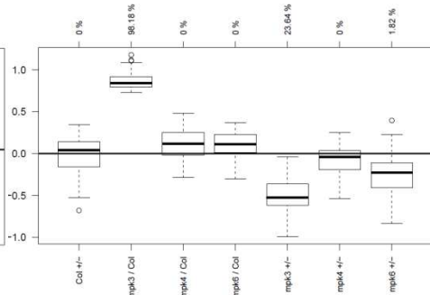
Cluster 14 / 55 genes
