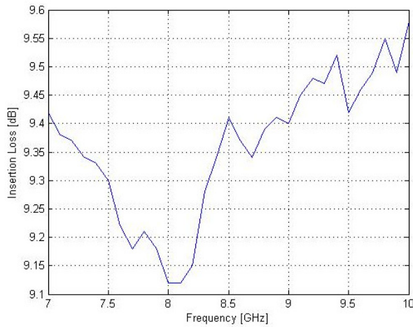
Fig. 7: Insertion Loss vs. Carrier Frequency
