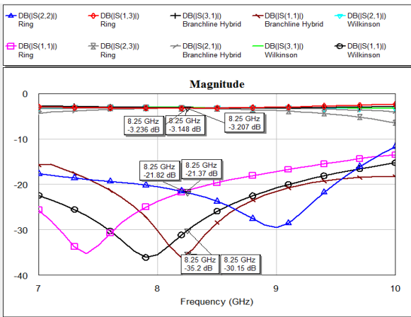
Fig. 1(a) Amplitude response of the three couplers
