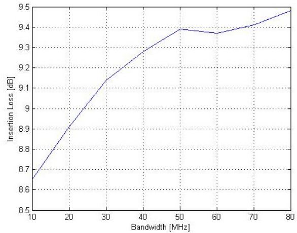
Fig. 9: Insertion Loss vs. Baseband Bandwidth
