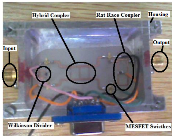
Fig. 6: Fabricated Modulator on Arlon's AD 450 PCB
