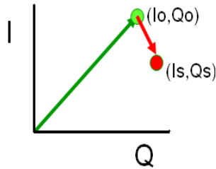
Fig. 12: EVM description
