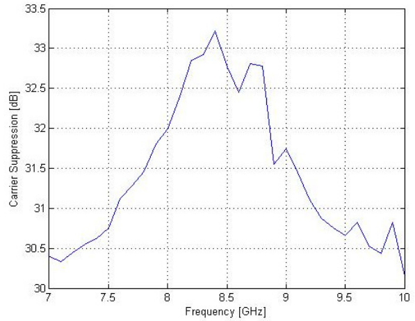
Fig. 8: Carrier Suppression vs. Carrier frequency
