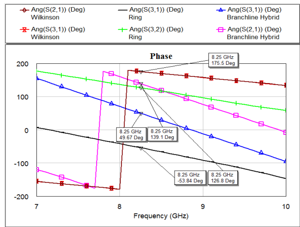
Fig. 1(b): Phase response of the three couplers
