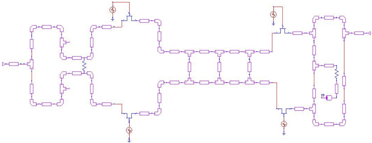
Fig. 2: Schematic of the Modulator
