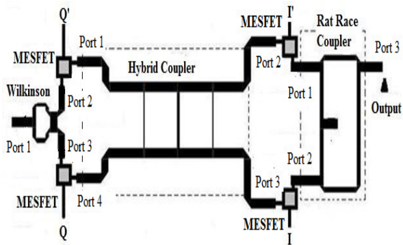
Fig. 4: Modulator Implementation
